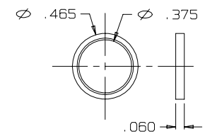
RING, STRAIN RELIEF TJSS-106-6
