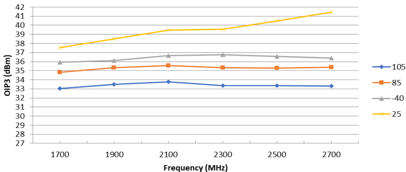
GRF2071 OIP3 vs. Frequency vs. Temperature
