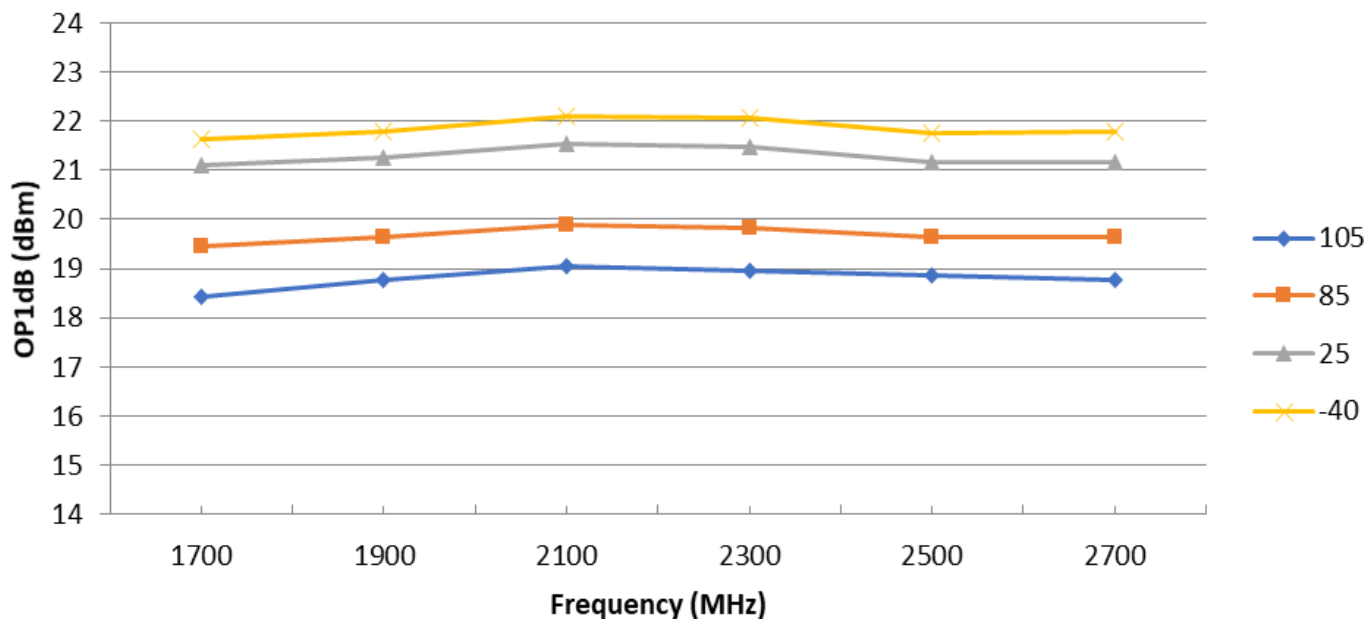
GRF2071 OP1dB vs. Frequency vs. Temperature
