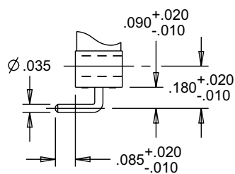
TERMINAL STYLE 7 RIGHT ANGLE PRINTED CIRCUIT PIN
