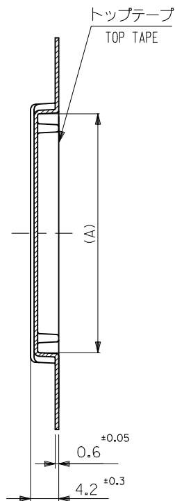
SECT:U-U
