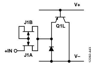
Figure 90. Overvoltage Protection Circuitry
