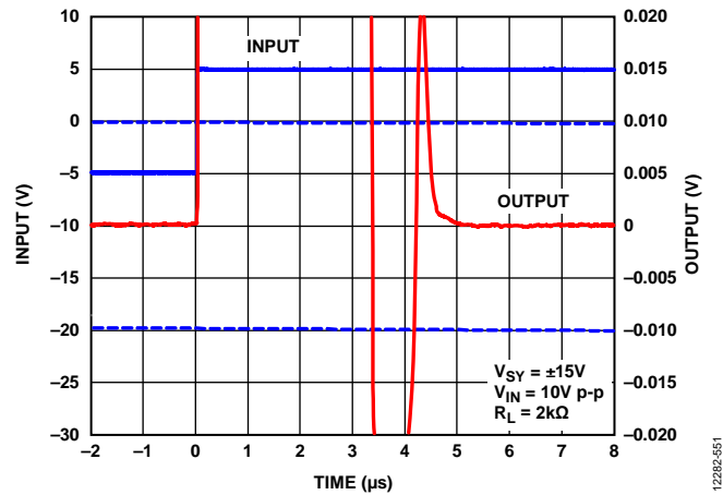
Figure 62. Positive Settling Time to 0.1%, V_{SY} = \pm 15 V
