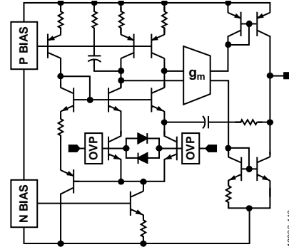
Figure 84. Conceptual Schematic
