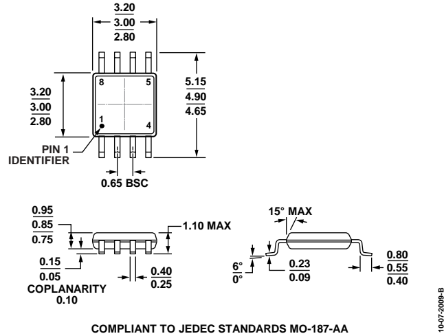
Figure 97. 8-Lead Mini Small Outline Package [MSOP] (RM-8) Dimensions shown in millimeters
