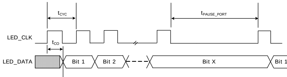
Figure 23 • Basic Serial LED Timing
