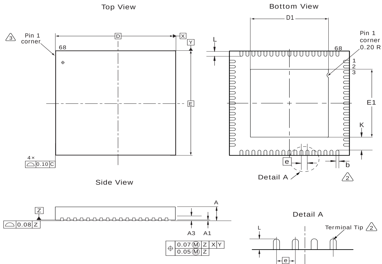
Figure 28 • Package Drawing
