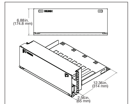
FiberExpress Ultra HD 4U Recessed Shelf
