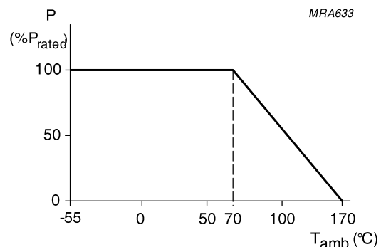
Fig. 6-2 Maximum dissipation ( P_{\max} ) in percentage of rated power as a function of the operating ambient temperature ( T_{\text{amb}} )
