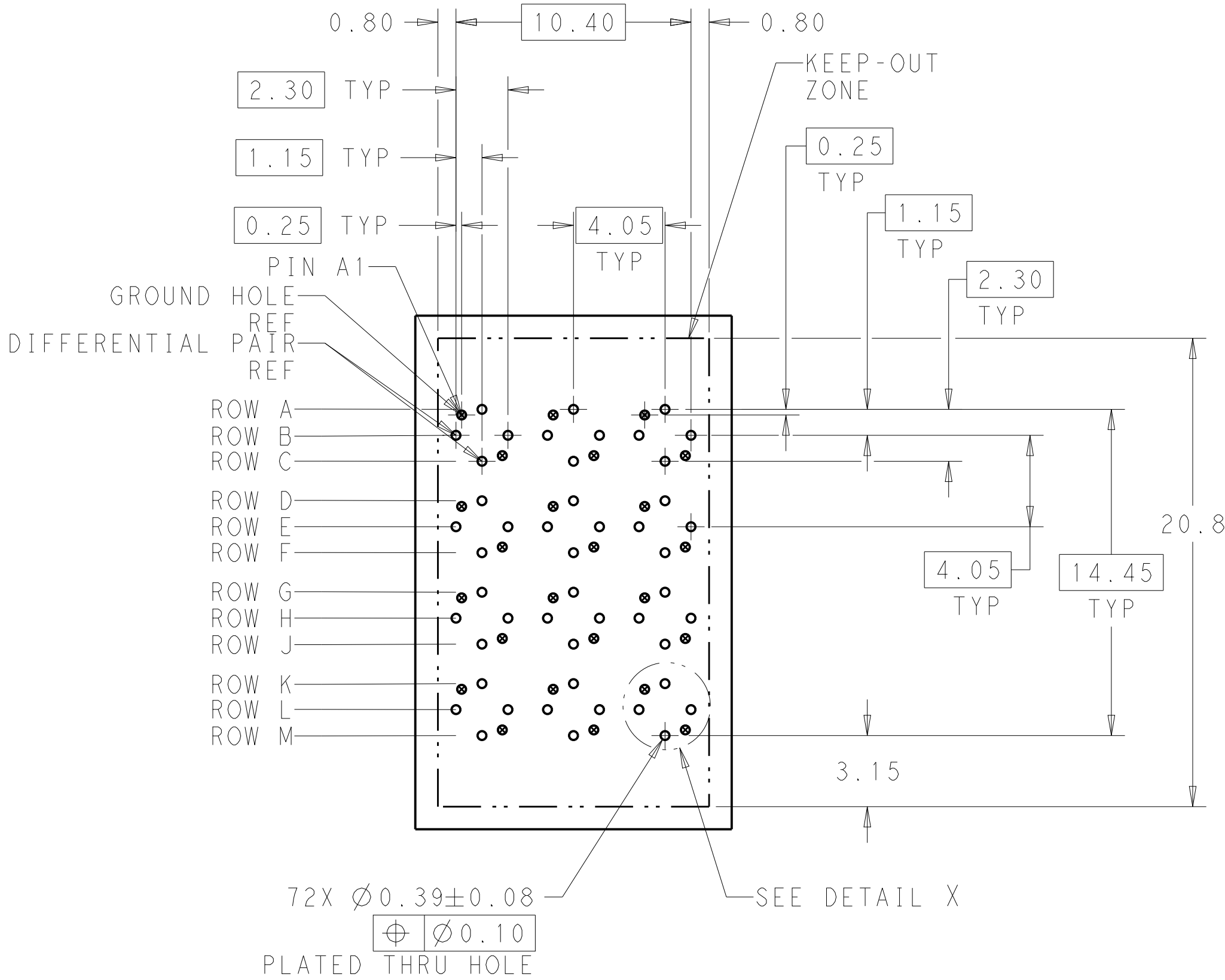
UNGUIDED BACKPLANE HOLE PATTERN (CONNECTOR SIDE)
