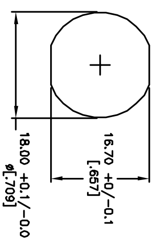
RECOMMEND PANEL MOUNTING
