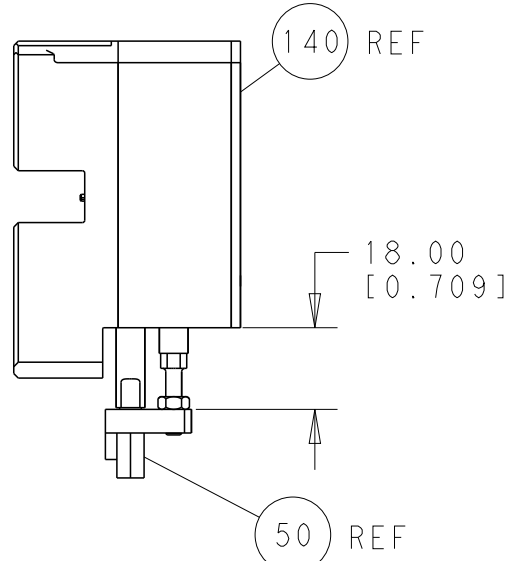
HOLDDOWN SET-UP
