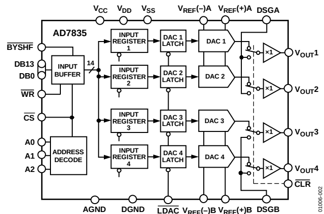
Figure 2. AD7835
