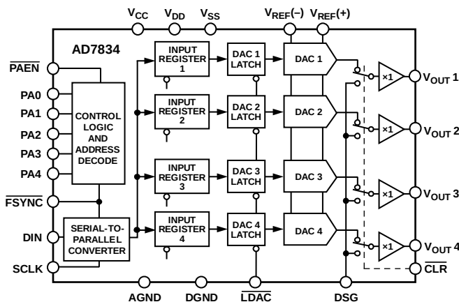
Figure 1. AD7834
