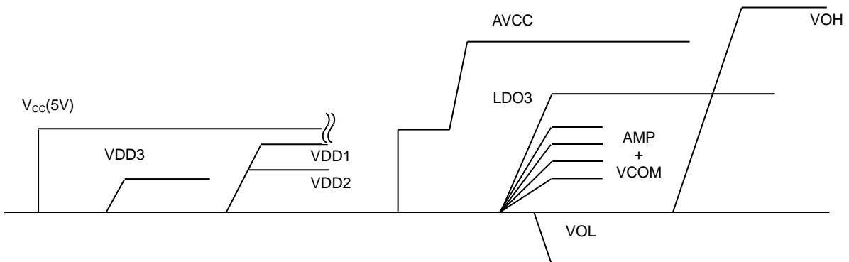
Figure 4. Sequence Chart
