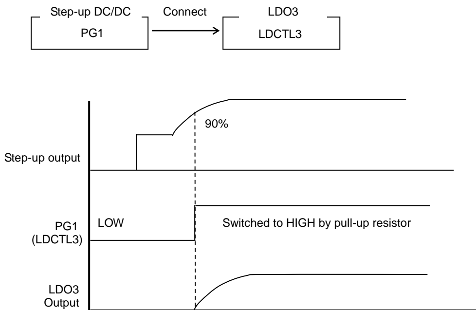
Figure 11. Typical Application of Control / Power Good Functions
