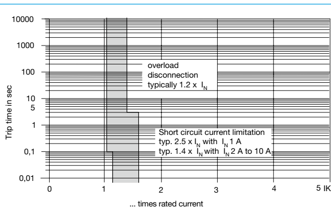
Time/current characteristic curve ( T_{amb} = 25\text{ °C} , U_B = \text{DC } 24\text{ V} )
