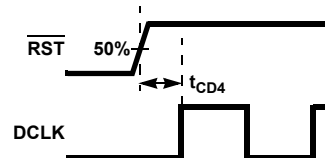
Figure 10. Decoder Timing
