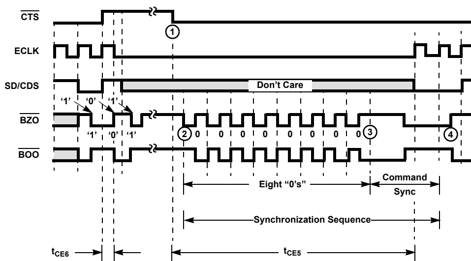
Figure 13. Encoder Operation
