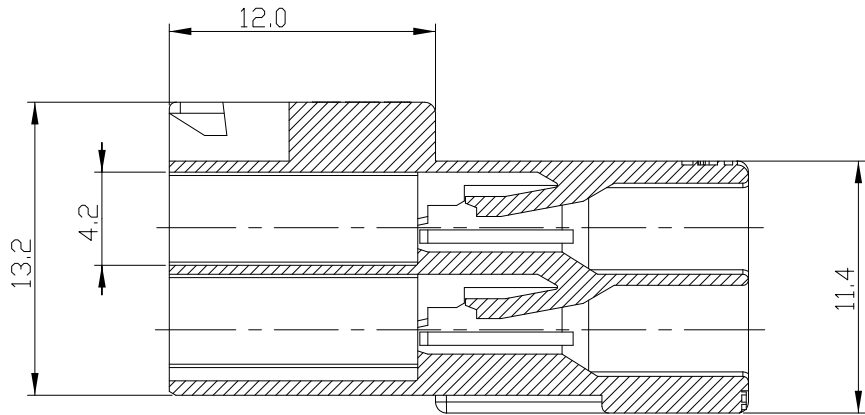
SECTION X-X
