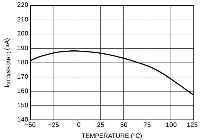
Figure 20. Current I_{NTC(SSTART)} Sourced from the Latch Pin, During Soft-Start
