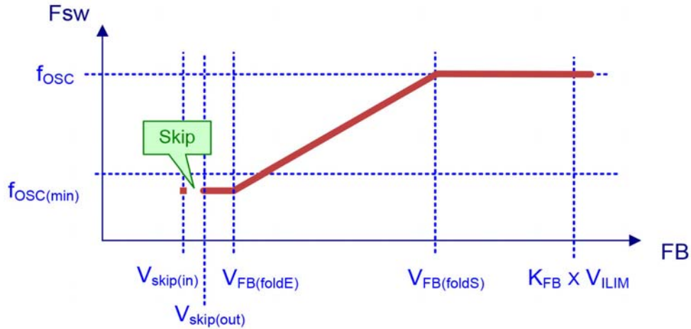
Figure 55. Frequency Foldback Mode Characteristic
