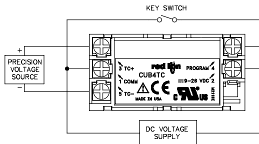
Voltage Calibration Wiring
