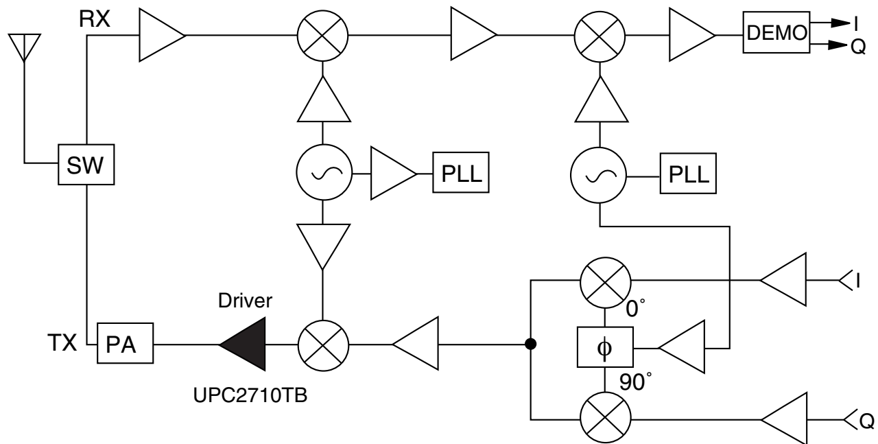
Example of 900 MHz Band Digital Cellular Telephone
