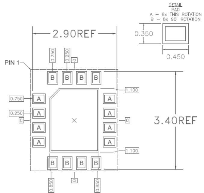
RECOMMENDED LAND PATTERN MASK
