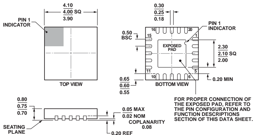
Figure 12. 20-Lead Lead Frame Chip Scale Package [LF CSP_WQ] 4 mm x 4 mm Body, Very Very Thin Quad (CP-20-6)
