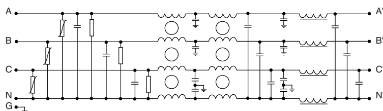
Circuit 2
