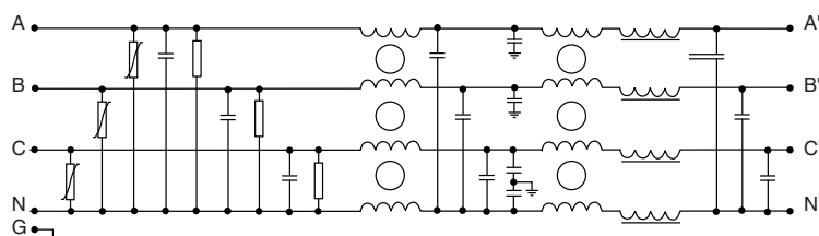
Circuit 1
