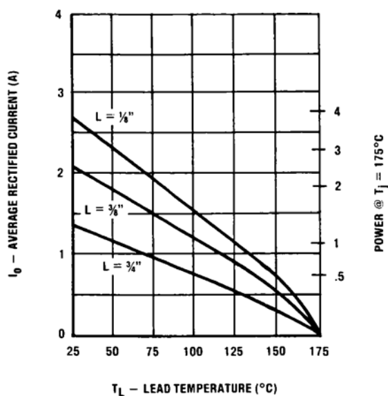
FIGURE 1 MAXIMUM CURRENT vs LEAD TEMPERATURE
