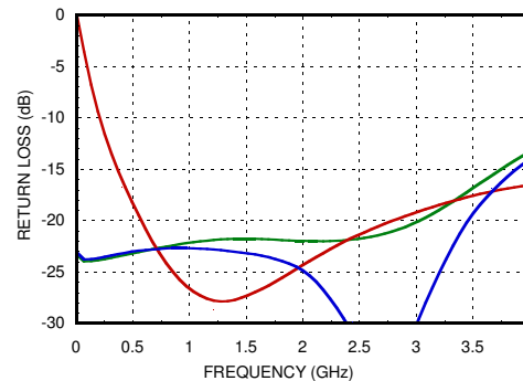
Return Loss
