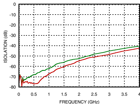
Isolation Between Ports RFC and RF1 / RF2
