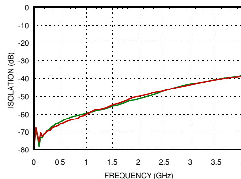
Isolation Between Ports RF1 and RF2
