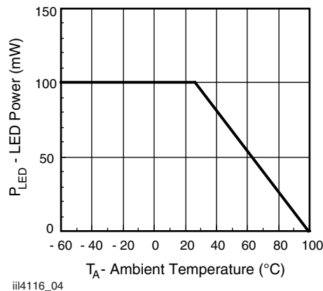
Fig. 5 - Maximum LED Power Dissipation
