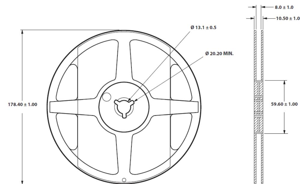
Figure 8: Reel Dimensions
