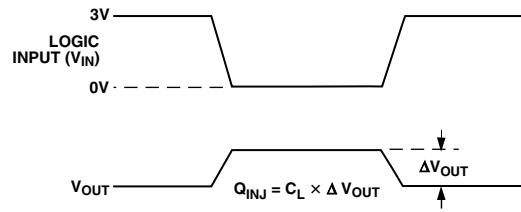
Test Circuit 7. Charge Injection
