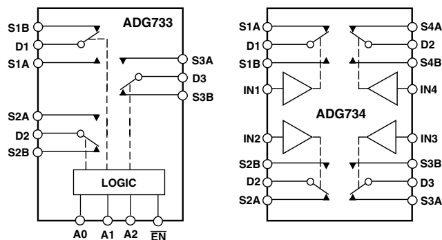
SWITCHES SHOWN FOR A "1" INPUT LOGIC
