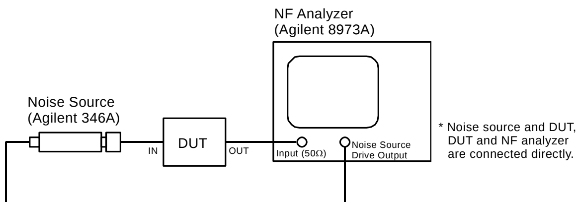
Measurement Setup
