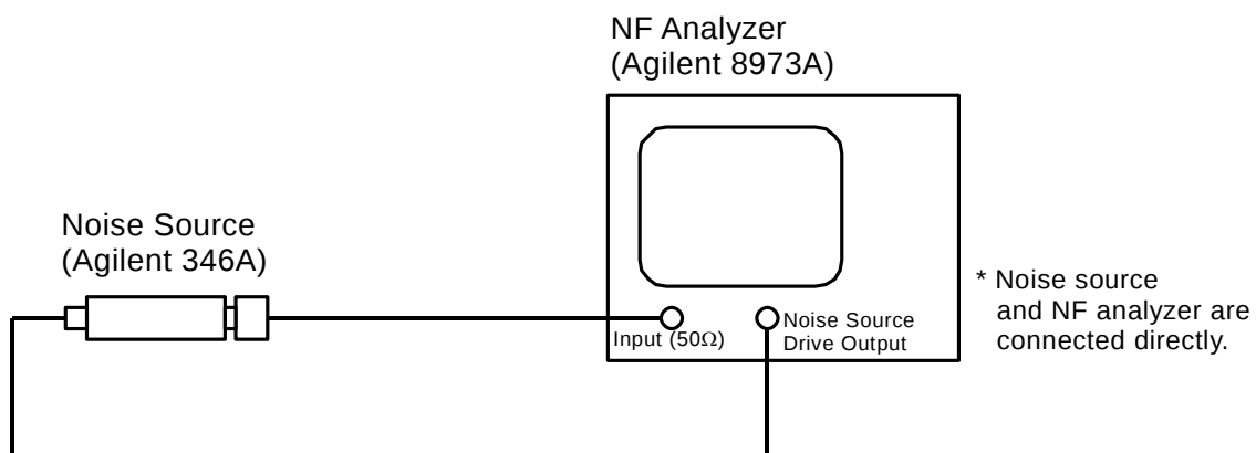
Calibration Setup
