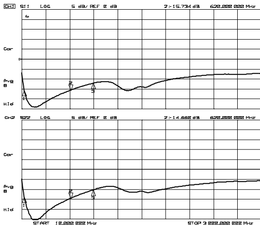
S11, S22
