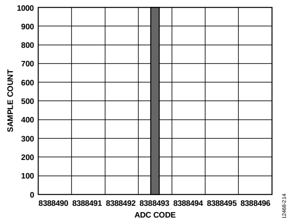
Figure 14. Histogram (Analog Input Buffers Enabled, V_{REF} = 5\text{ V} , Output Data Rate = 5 SPS)
