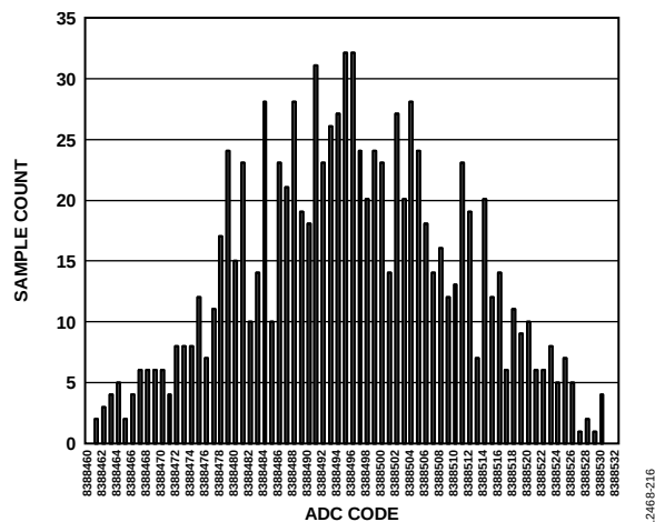
Figure 16. Histogram (Analog Input Buffers Enabled, V_{REF} = 5\text{ V} , Output Data Rate = 250 kSPS)
