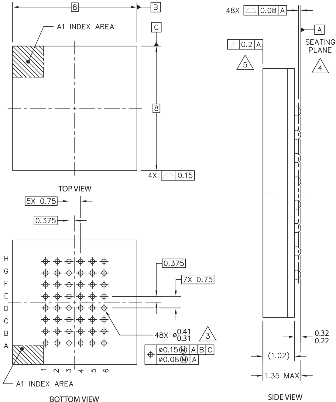
Figure 11 – 48-BGA Package Outline
