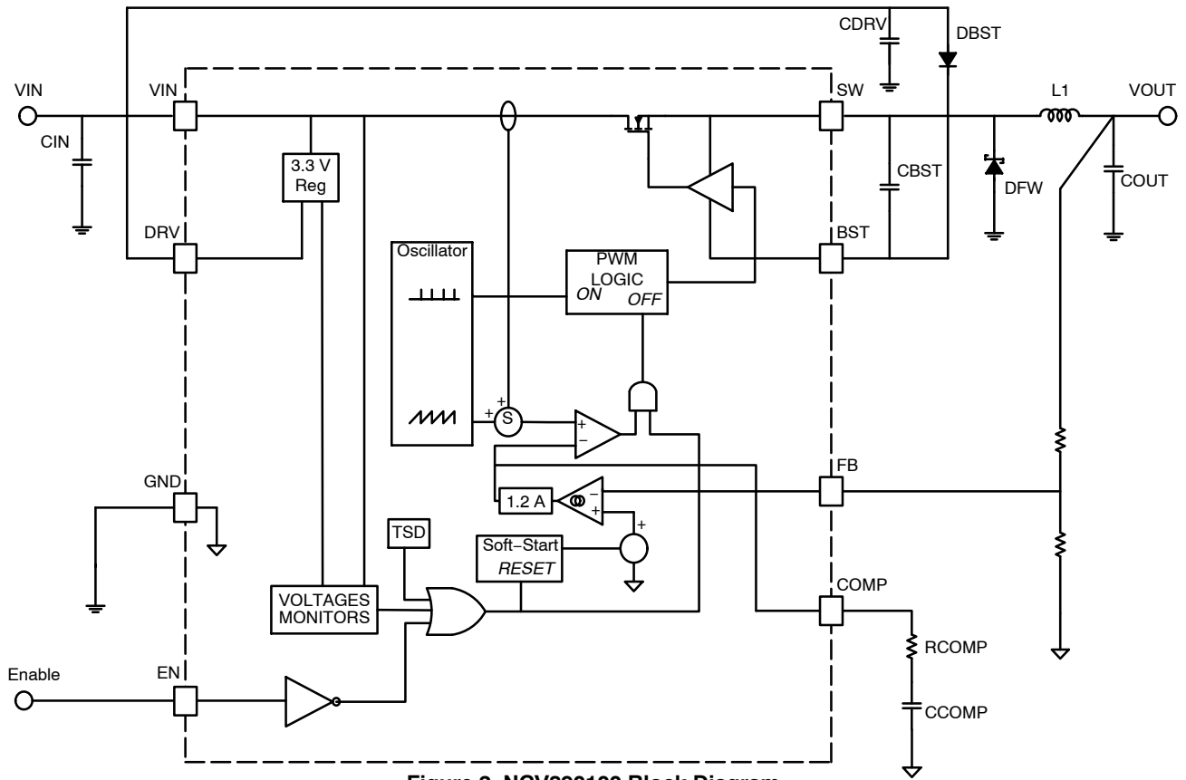
Figure 2. NCV890100 Block Diagram
