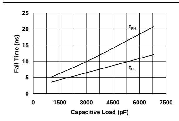
FIGURE 2-4: Fall Times vs. Capacitive Load.
