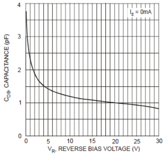
Fig. 4 Output Capacitance
