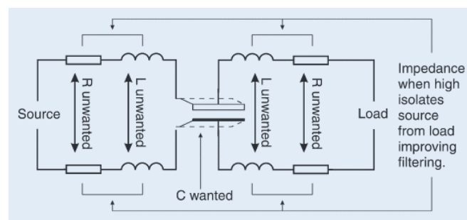
Figure 2: Network Capacitor
