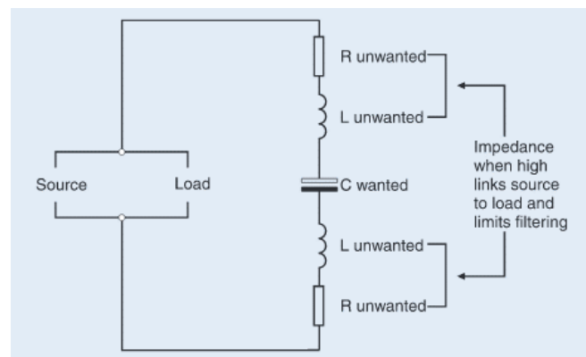
Figure 2: Network Capacitor
