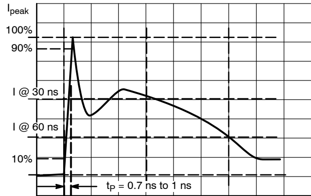
IEC61000-4-2 Waveform
