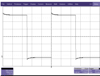
Overshoot
