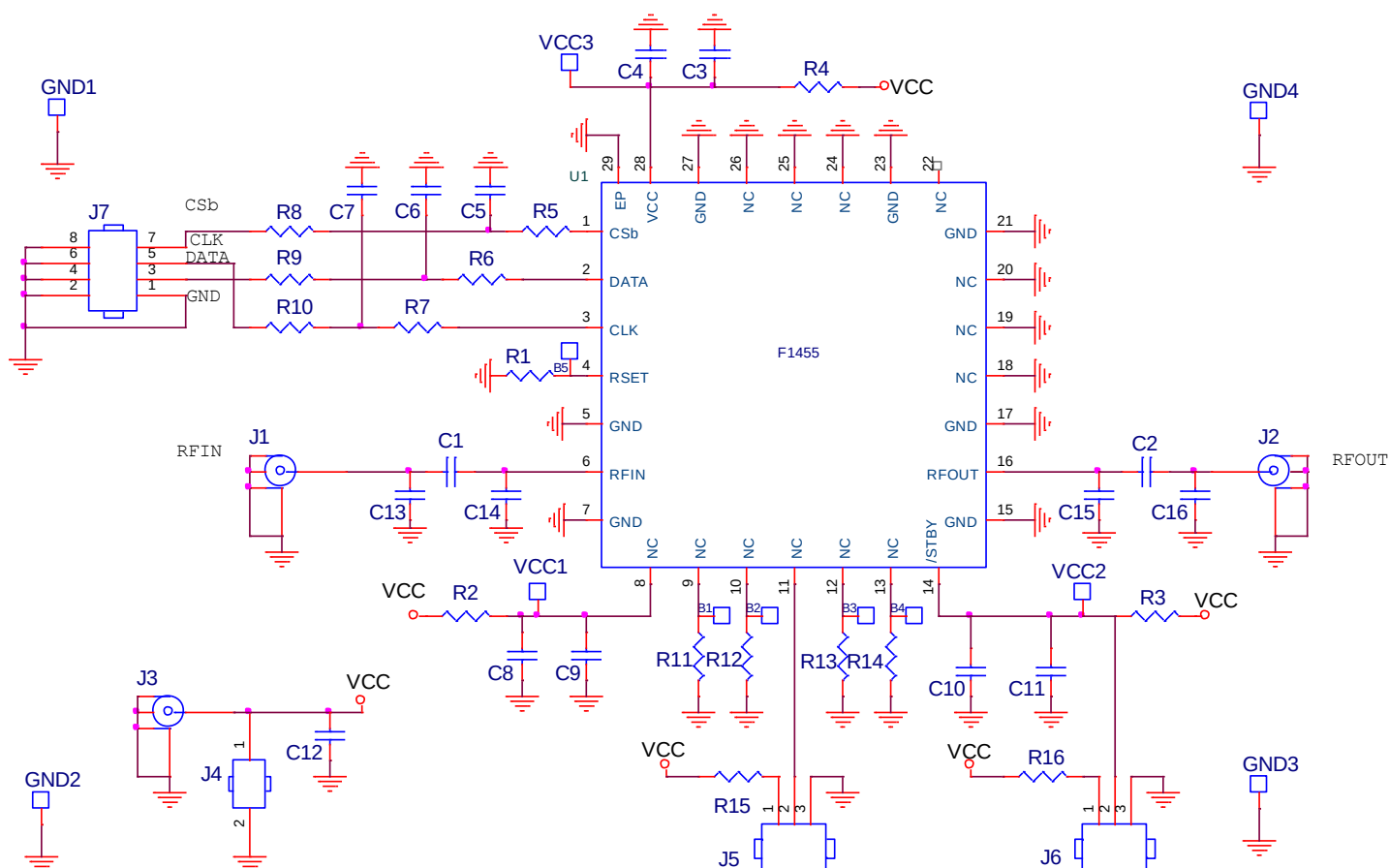
Figure 55. Electrical Schematic
