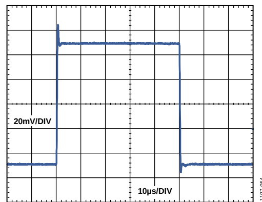
Figure 51. Small Signal Pulse Response ( G = 10 ), R_L = 2\text{ k}\Omega , C_L = 100\text{ pF}
