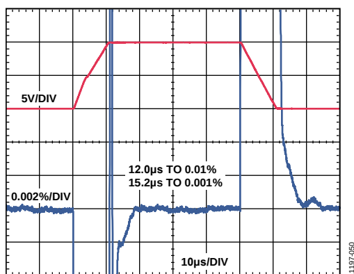
Figure 46. Large Signal Pulse Response and Settling Time ( G = 10 ), 10 V Step, V_S = \pm 15\text{ V} , R_L = 2\text{ k}\Omega , C_L = 100\text{ pF}
