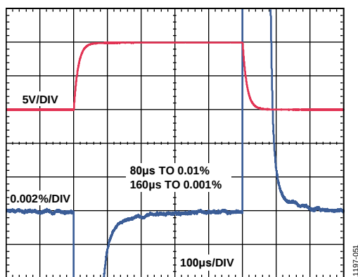
Figure 48. Large Signal Pulse Response and Settling Time ( G = 1000 ), 10 V Step, V_S = \pm 15\text{ V} , R_L = 2\text{ k}\Omega , C_L = 100\text{ pF}
