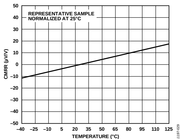
Figure 28. CMRR vs. Temperature ( G = 1 ), Normalized at 25°C
