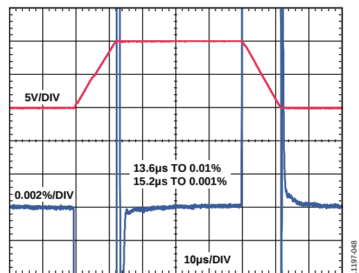
Figure 45. Large Signal Pulse Response and Settling Time ( G = 1 ), 10 V Step, V_S = \pm 15\text{ V} , R_L = 2\text{ k}\Omega , C_L = 100\text{ pF}
