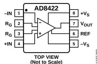
Figure 57. Pinout Diagram
