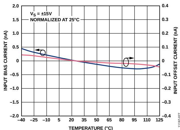
Figure 26. Input Bias Current and Input Offset Current vs. Temperature
