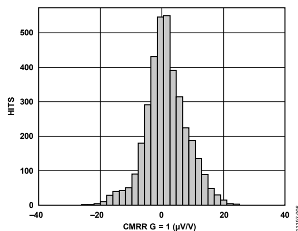
Figure 9. Typical Distribution of CMRR (G = 1)
