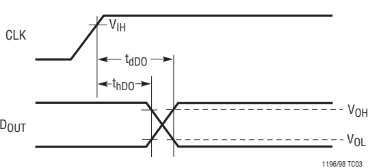
Voltage Waveform for D OUT Delay Time, t dDO , t hDO
