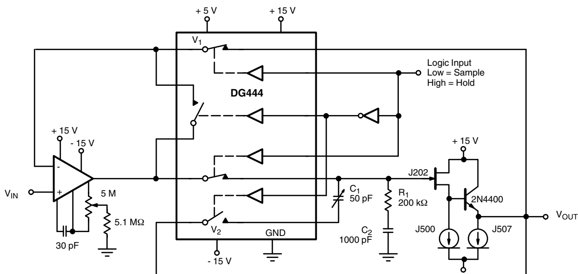
Figure 9. Precision Sample-and-Hold
