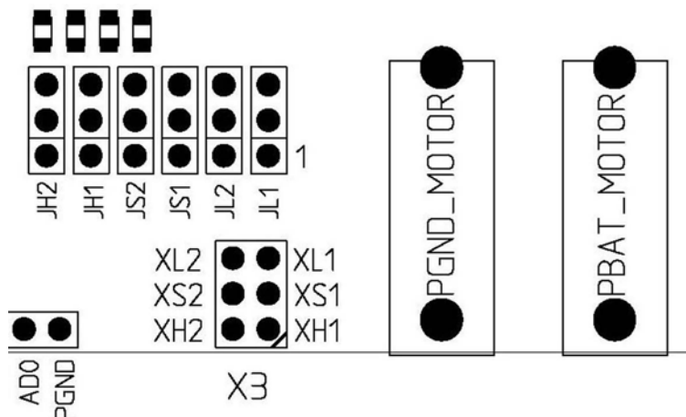
Figure 2-6. External H-bridge Connection
