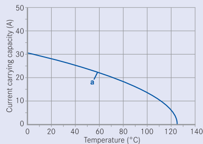
Curve a: 2.5 mm² Standard contact. wire gauge
