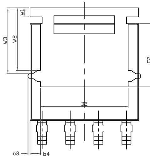
BACKSIDE VIEW(SINGLE)
